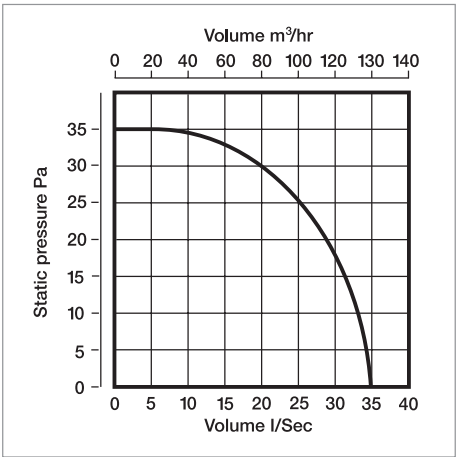
Performance - XFLP125
