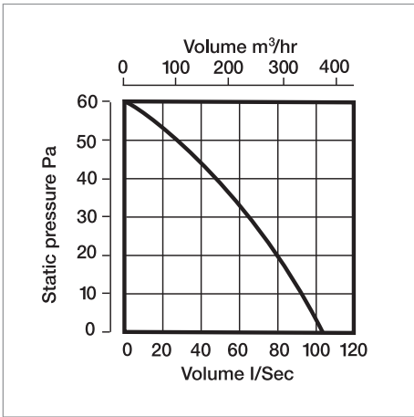
Performance - XFLP150
