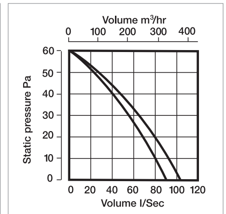
Performance - XF150
