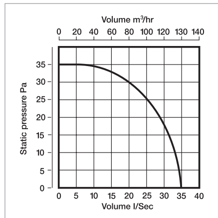
Performance - XF125
