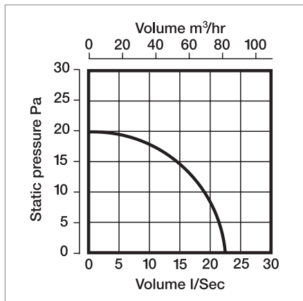
Performance - XF100
