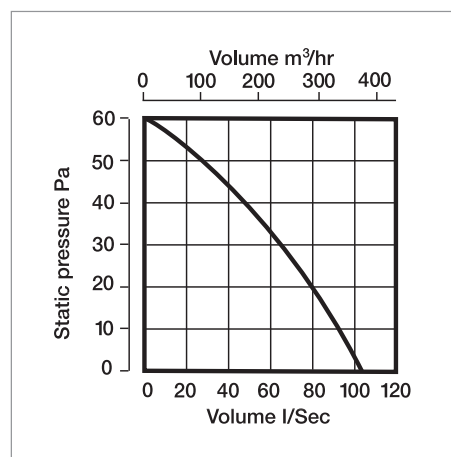
Performance - XFLP150
