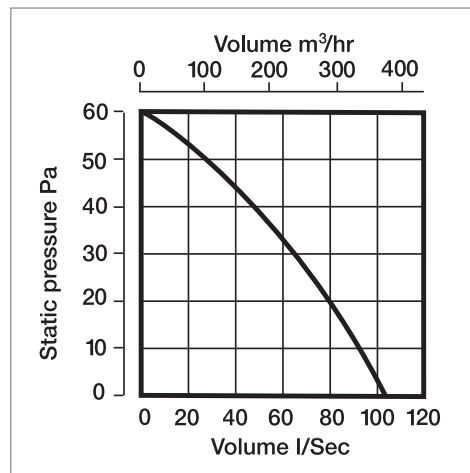
Performance - WF150
