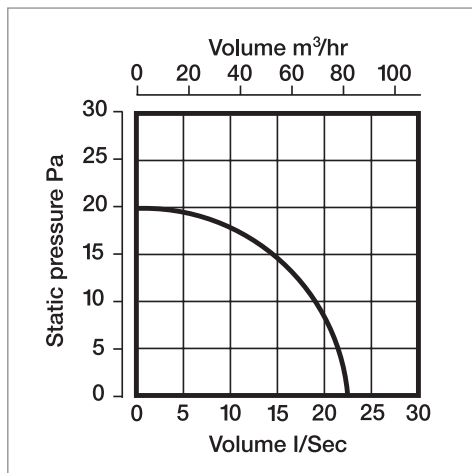
Performance - WF100
