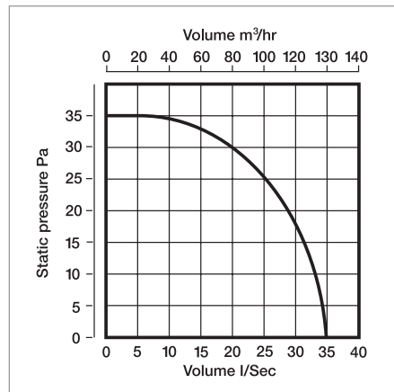
Performance - XF125
