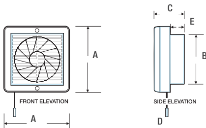
Dimensions - XF230/300
