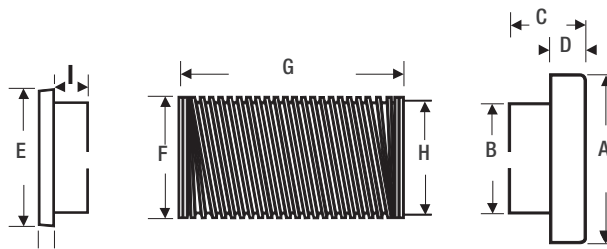
Dimensions - XPS230/300
