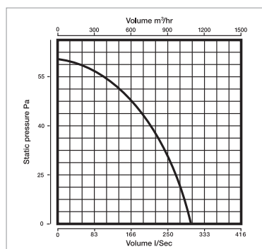
Performance - XFS300
