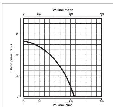
Performance - XFS230
