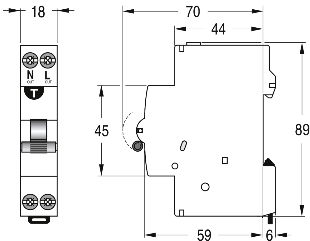
Dimension Diagram
