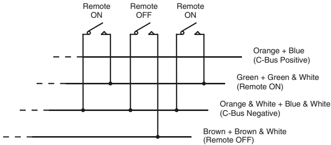
Figure 3 – Remote Override Connections
